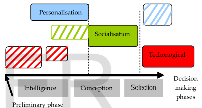
Fig. 2, The role of KS in the decision making process (Nicolas 2004).
